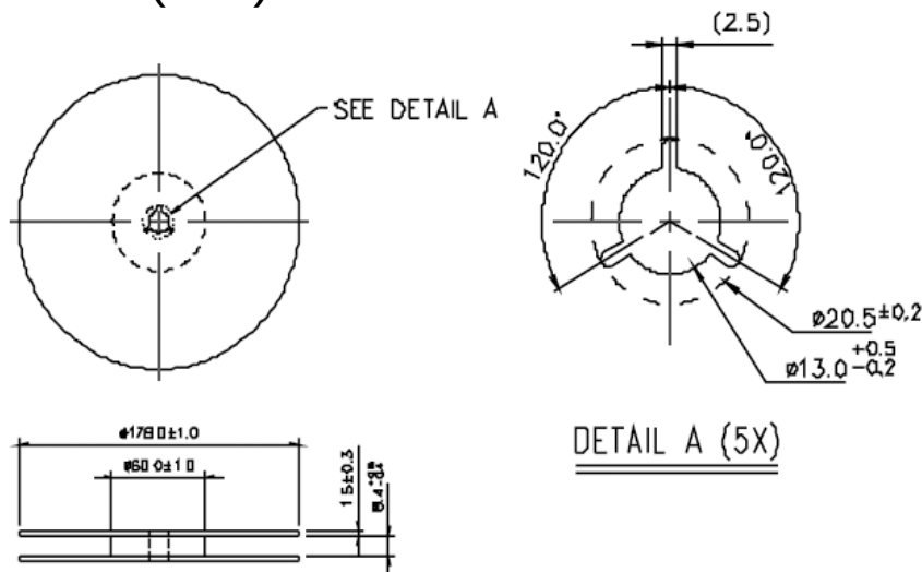
Tape Dimensions (mm):
